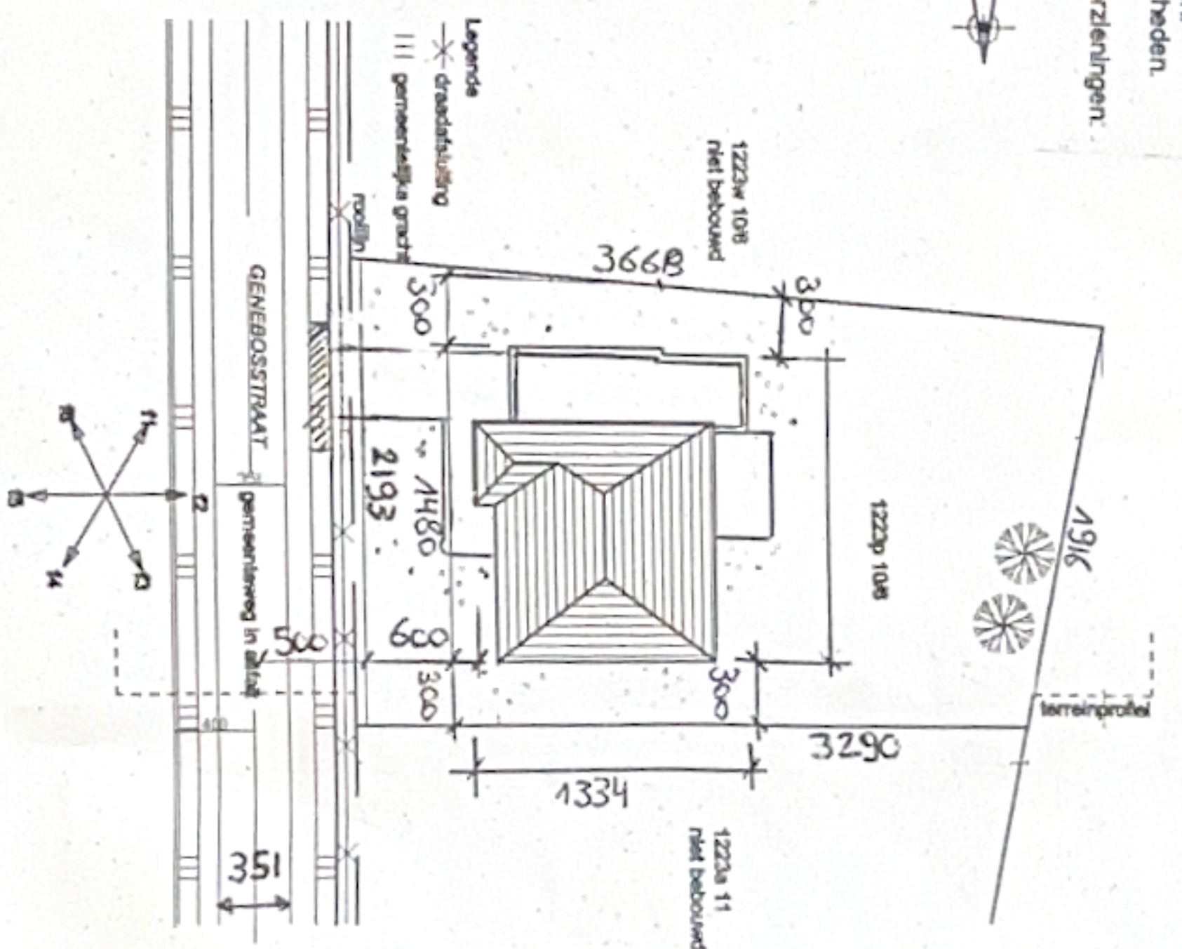
INPLANTINGSPLAN
